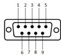
RS-232-DP9 Male
